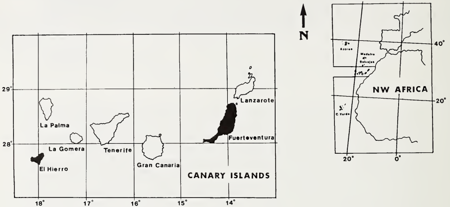
Fig. 1: Geographical location of the Canary Islands. Black areas: the islands covered by the study.
